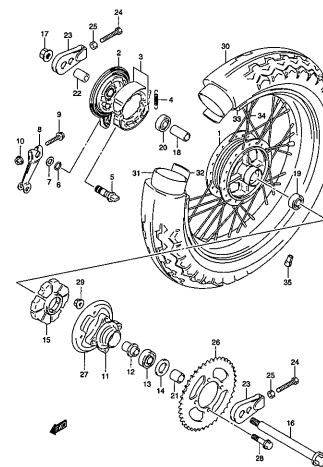
TU250XG9 000_056 REAR WHEEL
