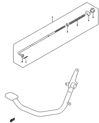
TU2500K9 000_044 REAR BRAKE ROD
