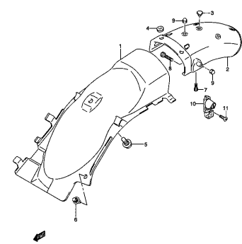
TU2500K9 000_041 REAR FENDER
