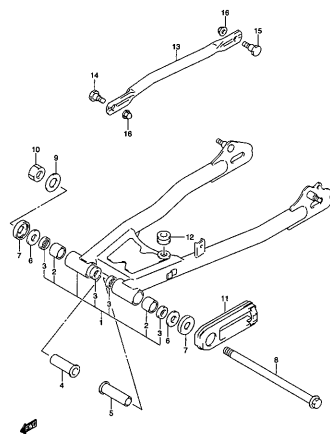
TU250XG9 000_054 REAR SWINGING ARM
