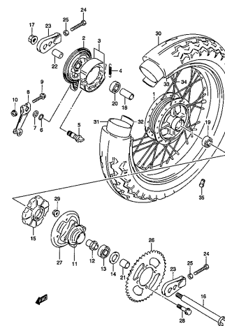
TU250XG9 000_057 REAR WHEEL
