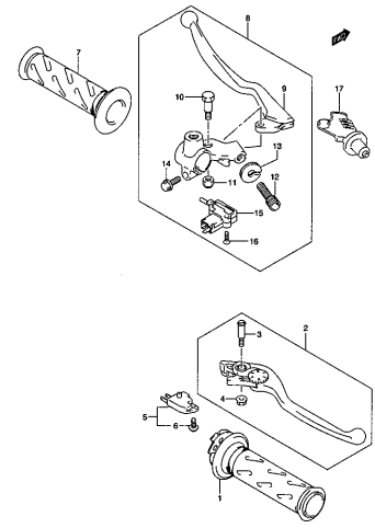
TU2500K9 000_040 HANDLE LEVER
